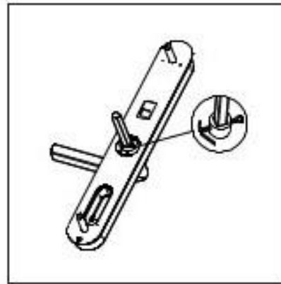
b Install the spindle into the handle hole in the front panel, and then insert the rod and fasten it;
