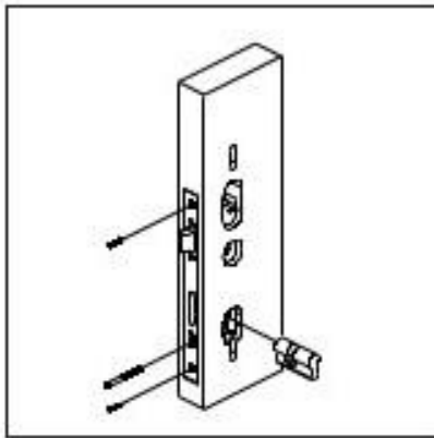
a Drill the holes on the door and then install the mortise into the door;
